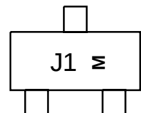
MARKING DIAGRAM & PIN ASSIGNMENT
